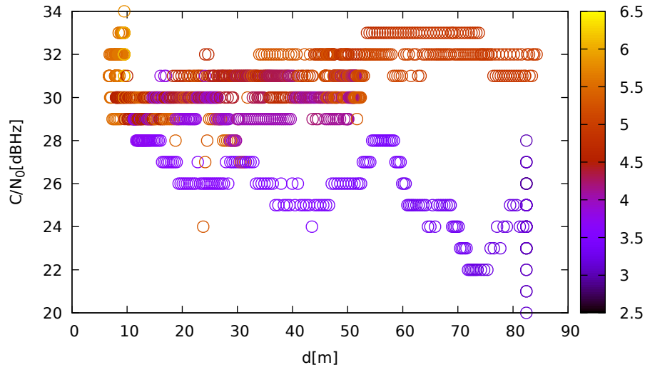
C/N 0 vs distance (ublox9 at C 3 for R14 at L2)
