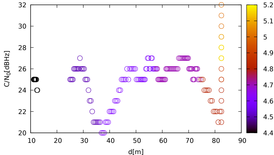
C/N 0 vs distance (ublox9 at C 3 for R15 at L2)
