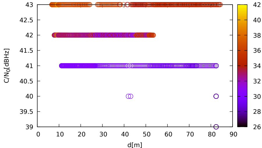
C/N 0 vs distance (ublox9 at C 3 for R21 at L2)
