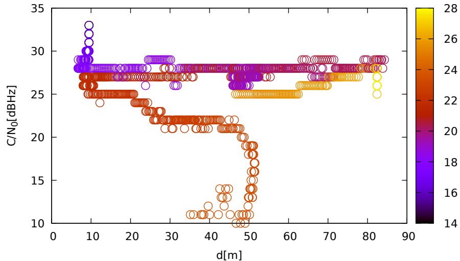
C/N 0 vs distance (ublox9 at C 3 for R23 at L2)
