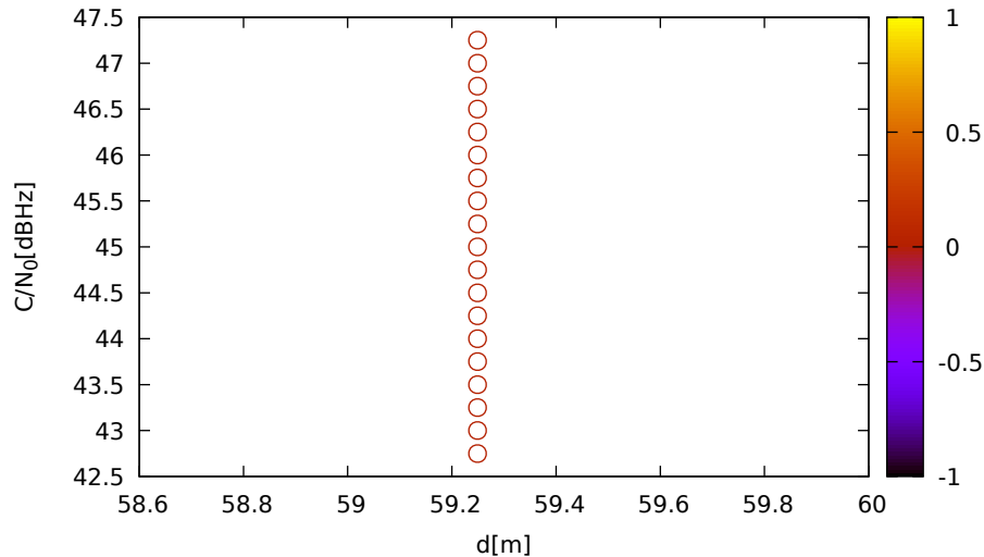
C/N 0 vs distance (JavadLSA at C 1 for E02 at L5)
