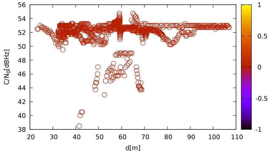
C/N 0 vs distance (JavadLSA at C 1 for E04 at L5)
