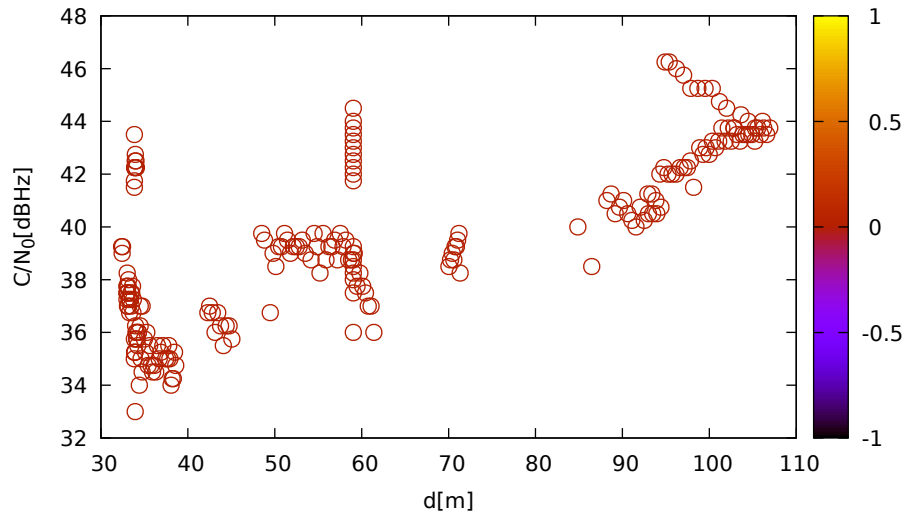
C/N 0 vs distance (JavadLSA at C 1 for E05 at L5)
