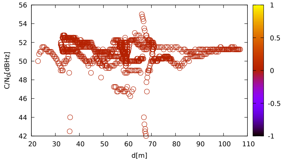
C/N 0 vs distance (JavadLSA at C 1 for E09 at L5)
