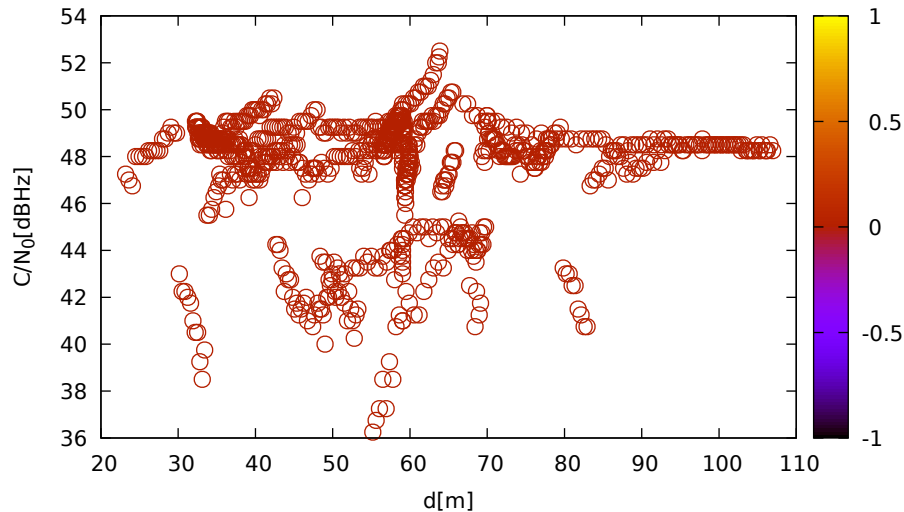
C/N 0 vs distance (JavadLSA at C 1 for E11 at L5)
