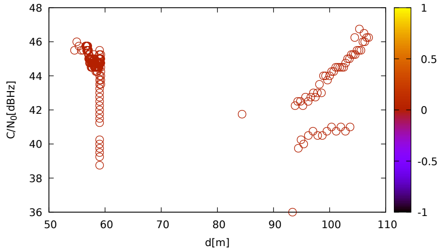
C/N 0 vs distance (JavadLSA at C 1 for E12 at L5)
