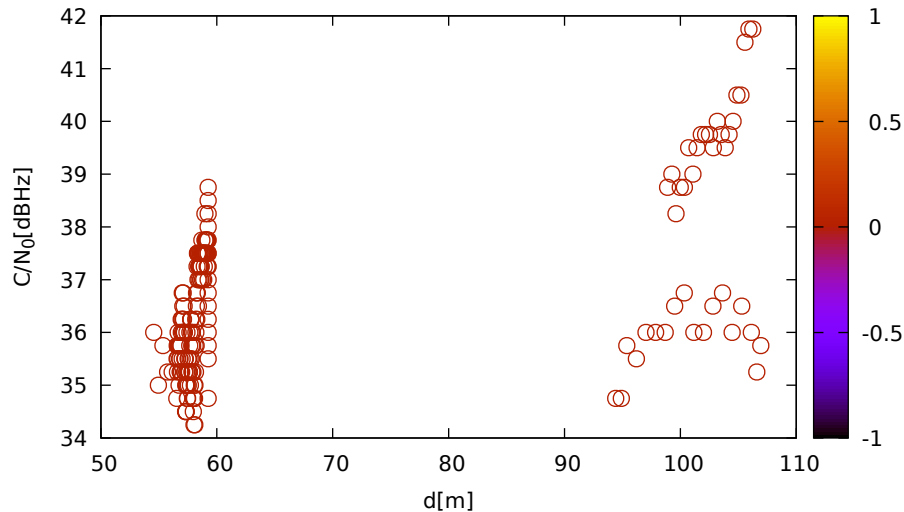
C/N 0 vs distance (JavadLSA at C 1 for E19 at L5)
