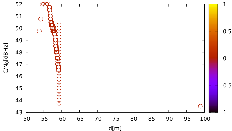
C/N 0 vs distance (JavadLSA at C 1 for E30 at L5)
