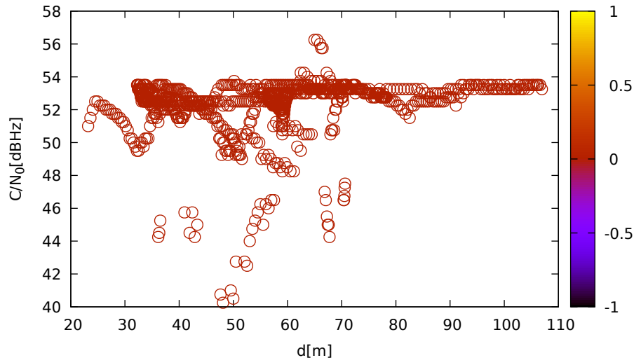
C/N 0 vs distance (JavadLSA at C 1 for E36 at L5)
