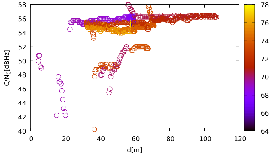
C/N 0 vs distance (JavadLSA at C 1 for G01 at L5)
