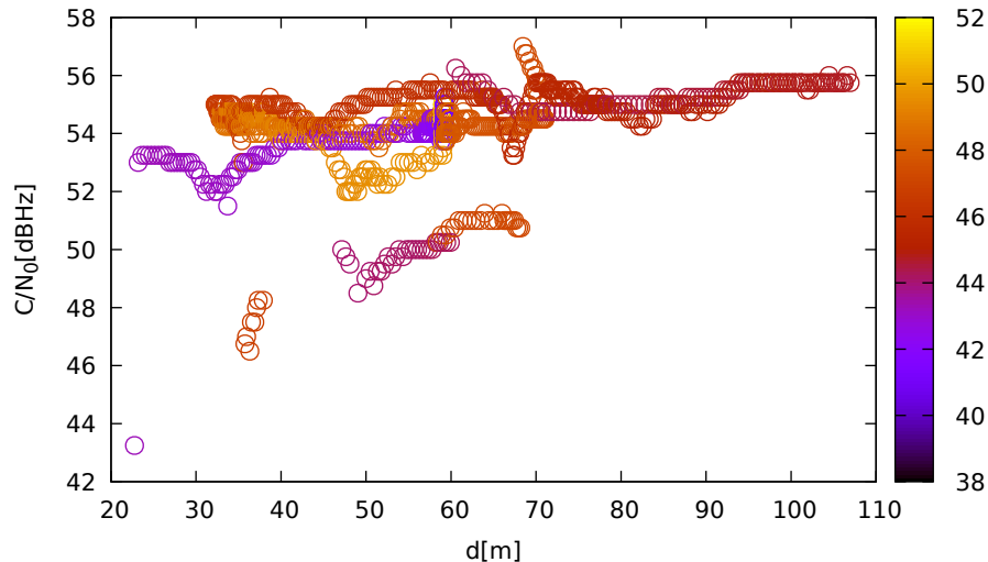
C/N 0 vs distance (JavadLSA at C 1 for G03 at L5)
