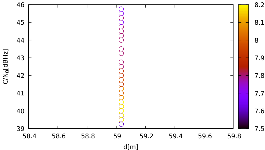
C/N 0 vs distance (JavadLSA at C 1 for G04 at L5)
