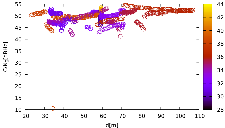
C/N 0 vs distance (JavadLSA at C 1 for G08 at L5)
