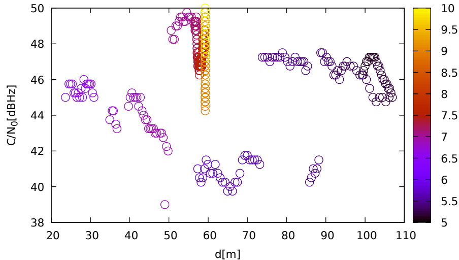
C/N 0 vs distance (JavadLSA at C 1 for G10 at L5)
