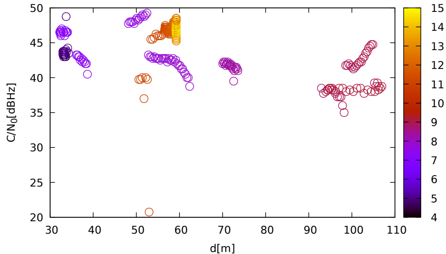
C/N 0 vs distance (JavadLSA at C 1 for G27 at L5)
