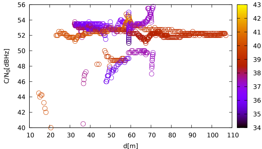
C/N 0 vs distance (JavadLSA at C 1 for G32 at L5)
