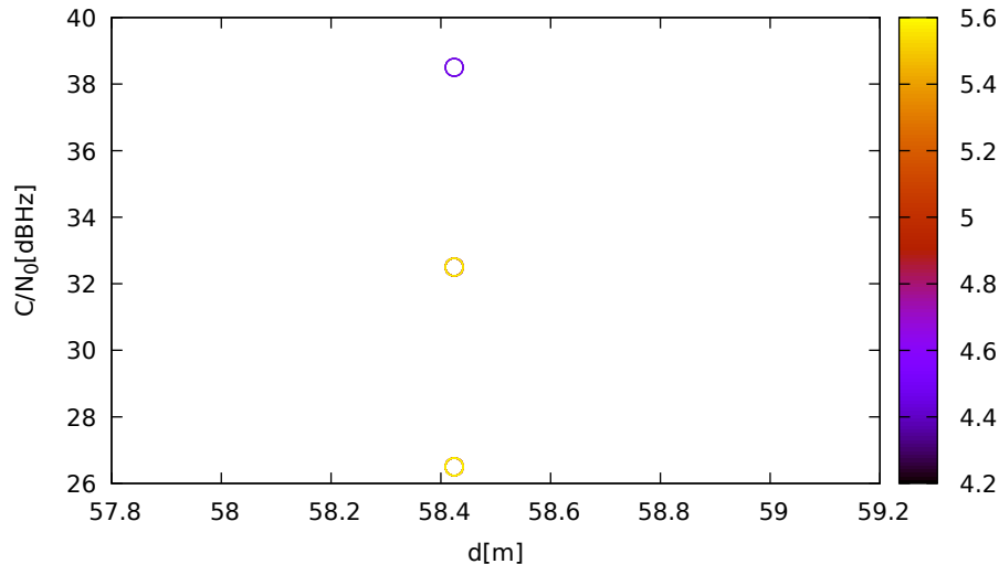
C/N 0 vs distance (LeicaGS15 at C 1 for E02 at L5)
