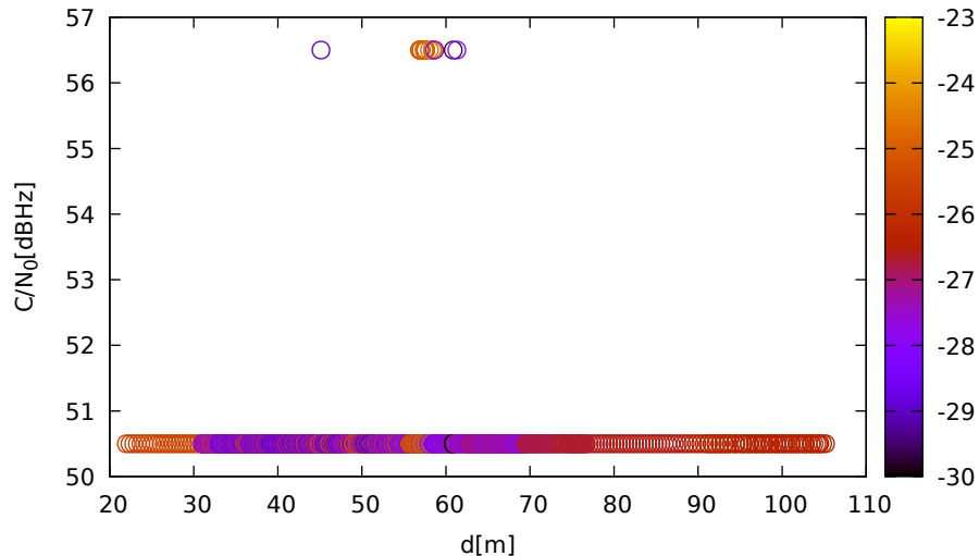
C/N 0 vs distance (LeicaGS15 at C 1 for E04 at L5)
