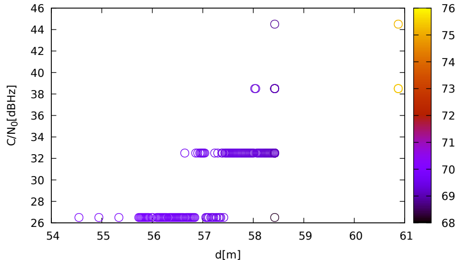
C/N 0 vs distance (LeicaGS15 at C 1 for E05 at L5)
