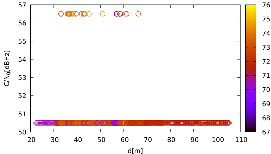
C/N 0 vs distance (LeicaGS15 at C 1 for E09 at L5)
