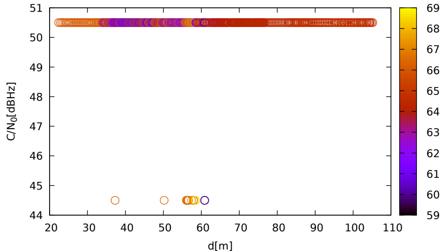
C/N 0 vs distance (LeicaGS15 at C 1 for E11 at L5)
