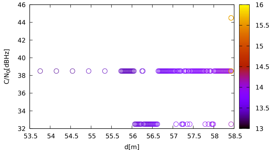
C/N_0 vs distance (LeicaGS15 at C_1 for E12 at L5)
