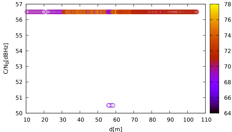
C/N 0 vs distance (LeicaGS15 at C 1 for G01 at L5)
