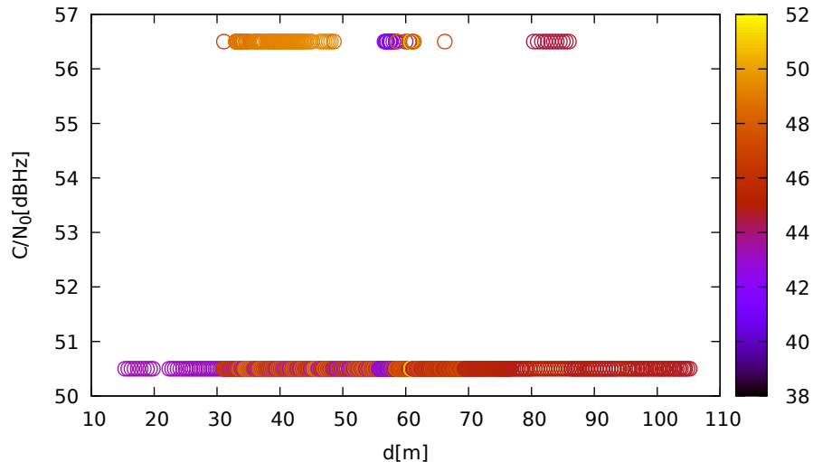
C/N 0 vs distance (LeicaGS15 at C 1 for G03 at L5)
