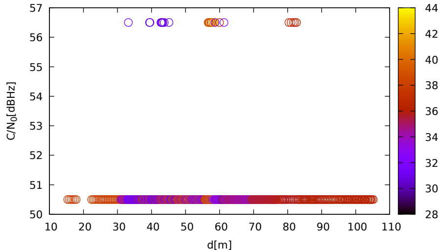
C/N 0 vs distance (LeicaGS15 at C 1 for G08 at L5)
