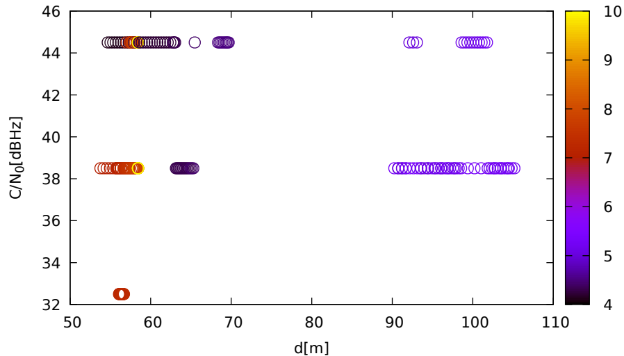
C/N 0 vs distance (LeicaGS15 at C 1 for G10 at L5)
