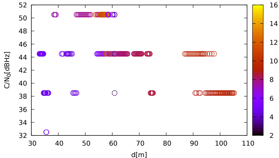
C/N 0 vs distance (LeicaGS15 at C 1 for G27 at L5)
