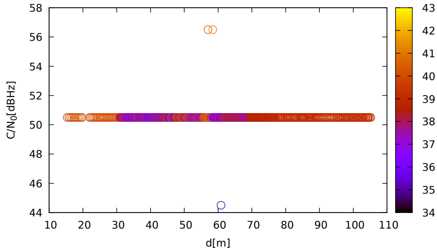
C/N 0 vs distance (LeicaGS15 at C 1 for G32 at L5)
