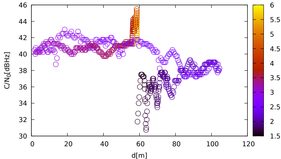
C/N 0 vs distance (LeicaGS18 at C 1 for E02 at L5)
