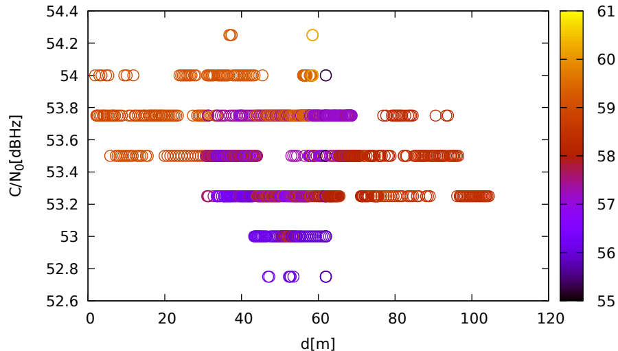
C/N 0 vs distance (LeicaGS18 at C 1 for E04 at L5)
