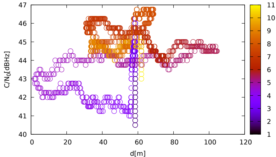
C/N 0 vs distance (LeicaGS18 at C 1 for E05 at L5)
