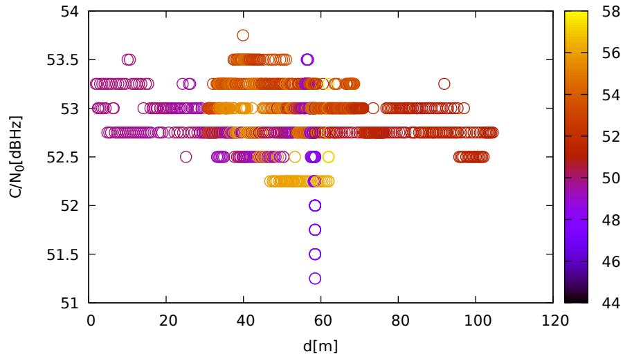
C/N 0 vs distance (LeicaGS18 at C 1 for E09 at L5)
