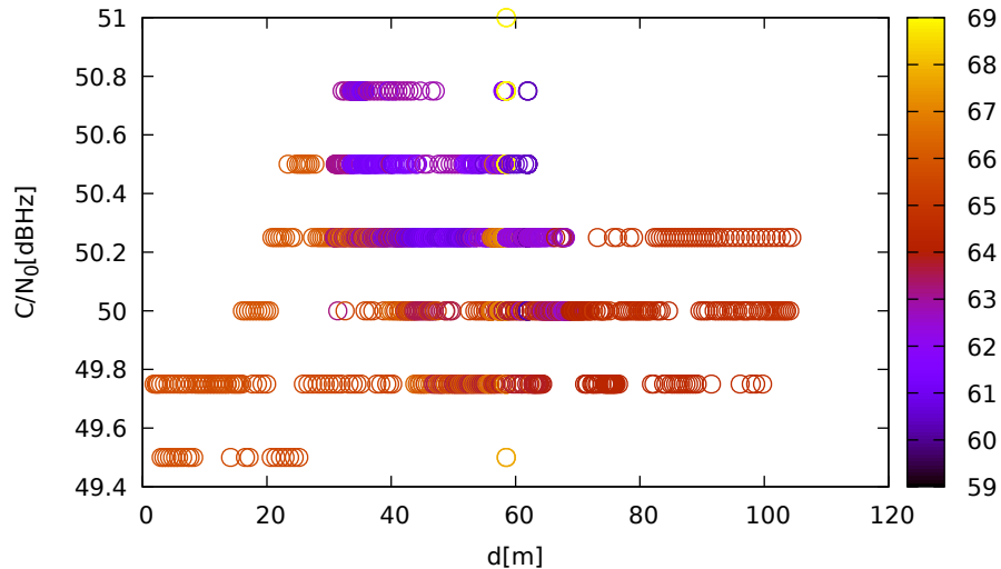
C/N 0 vs distance (LeicaGS18 at C 1 for E11 at L5)
