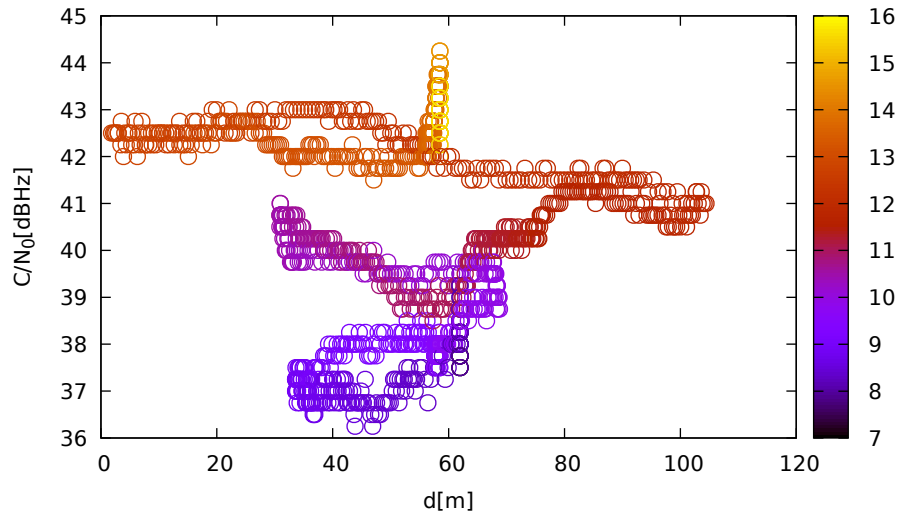
C/N 0 vs distance (LeicaGS18 at C 1 for E12 at L5)
