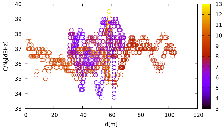
C/N 0 vs distance (LeicaGS18 at C 1 for E19 at L5)
