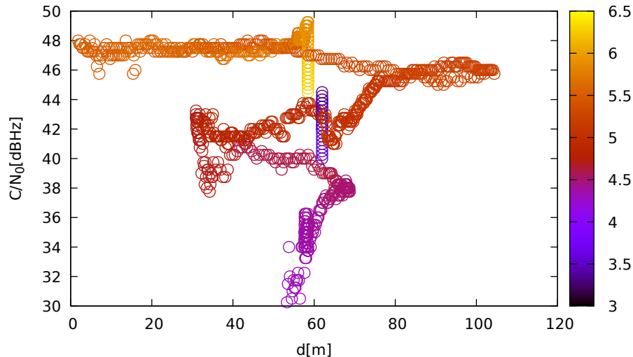
C/N_0 vs distance (LeicaGS18 at C_1 for E30 at L5)
