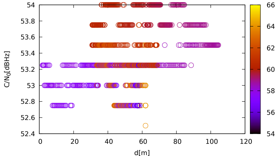
C/N 0 vs distance (LeicaGS18 at C 1 for E36 at L5)
