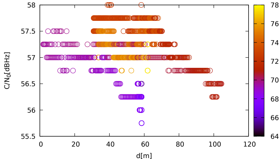
C/N 0 vs distance (LeicaGS18 at C 1 for G01 at L5)
