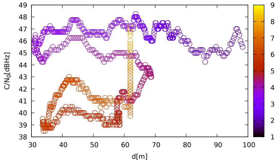
C/N 0 vs distance (LeicaGS18 at C 1 for G04 at L5)
