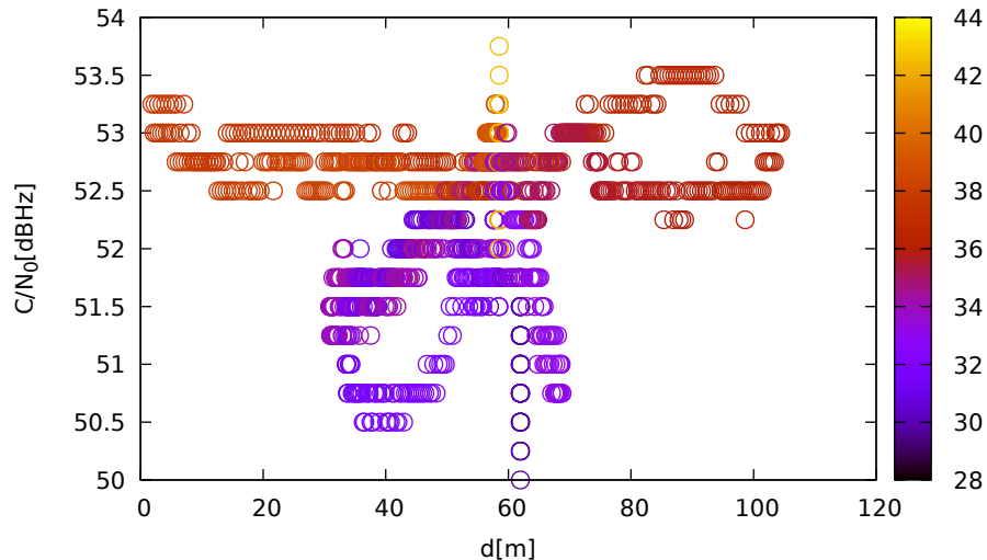
C/N 0 vs distance (LeicaGS18 at C 1 for G08 at L5)
