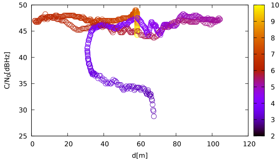
C/N 0 vs distance (LeicaGS18 at C 1 for G10 at L5)
