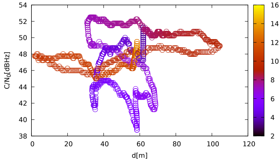
C/N 0 vs distance (LeicaGS18 at C 1 for G27 at L5)
