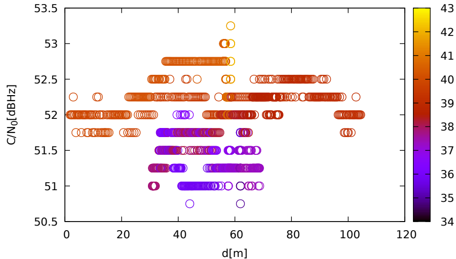
C/N 0 vs distance (LeicaGS18 at C 1 for G32 at L5)
