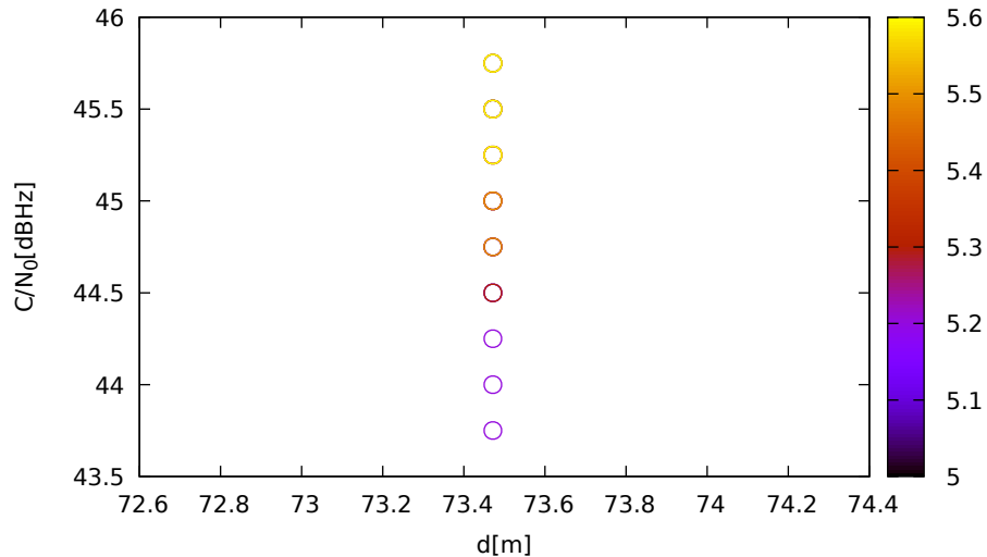
C/N 0 vs distance (JavadLSA at C 2 for E02 at L5)
