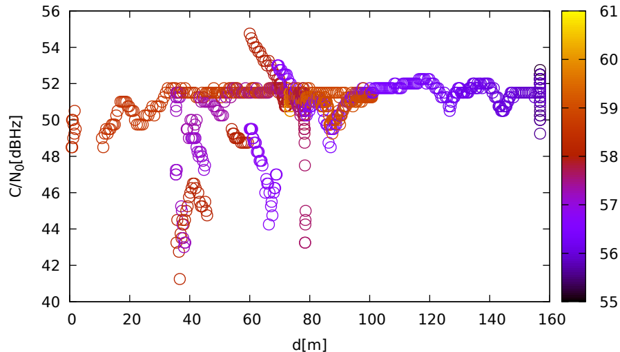
C/N 0 vs distance (JavadLSA at C 2 for E04 at L5)
