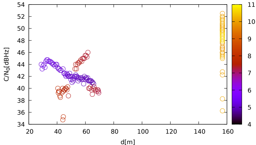
C/N 0 vs distance (JavadLSA at C 2 for E05 at L5)
